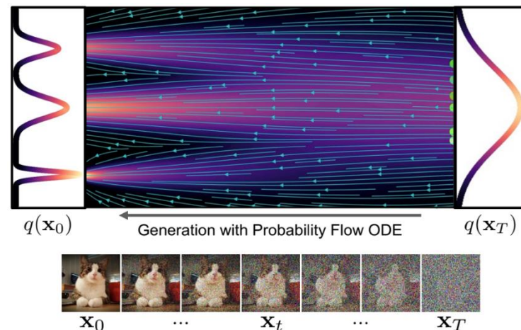
Probability Flow ODE:
